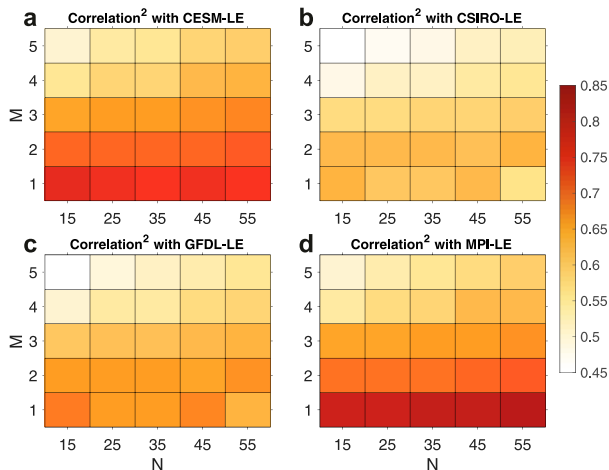
FIG. 16. Global mean of gridpoint squared correlation between ( \mathbf{X}_{LFP} ), computed entirely from the HadCRUT4 observational product, and ( \mathbf{X}_{S/NP} ), computed from four different large ensembles, over the time period 1930–2019 (excluding the micro-initialization spinup period), as a function of the number M of LFPs included and the number N of EOFs retained in the observational LFP filtering. The values of M and N used in the S/NP filtering are given in the caption of Fig. 15.
