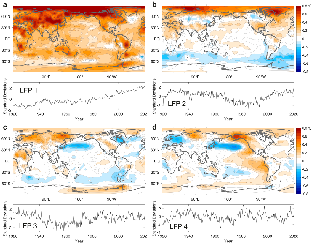
FIG. 12. Low-frequency patterns (LFPs) of seasonal surface temperature anomalies, and their time evolution in standard deviation anomalies, from the infilled HadCRUT4 (Cowan and Way 2014) observational product over the time period 1920–2019, with N = 25 EOFs retained.
