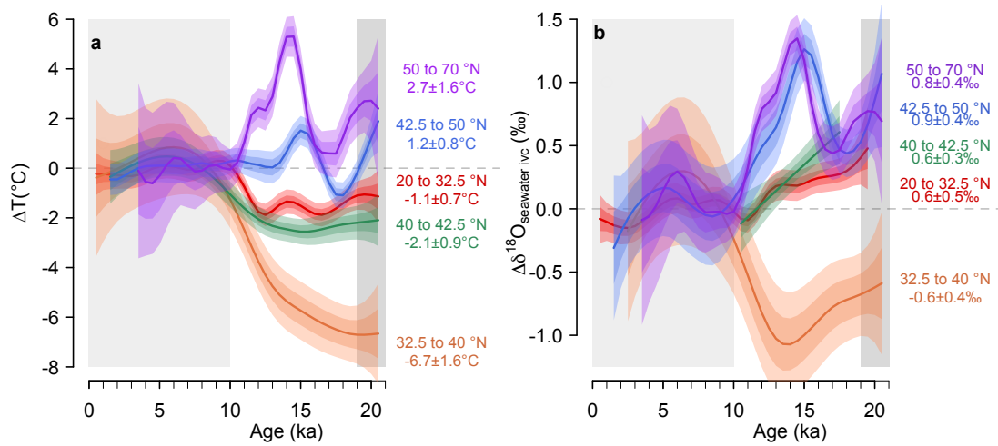
Figure S4: Latitudinally binned deglacial changes in SST (a) and \delta^{18}\text{O} of seawater (b). (a) At each site Mg/Ca and/or \text{U}^{\text{K}^*}_{37} SSTs were converted to a difference from Holocene (0-10 ka, light grey box) and binned by latitude. (b) \delta^{18}\text{O} of seawater, derived from paired measurements of Mg/Ca and \delta^{18}\text{O}_{\text{calcite}} and corrected for changes in global ice volume, was converted to a difference from Holocene and binned by latitude. The latitudinally binned SST and \delta^{18}\text{O}_{\text{seawater}} data were modelled as a function of time using a generalised additive model (GAM), with the 68% and 95% Bayesian credible intervals shown (161, 163). For each latitudinal SST and \delta^{18}\text{O}_{\text{seawater}} bin, the LGM (19-21 ka, dark grey box) value is given with the 95% confidence interval.
