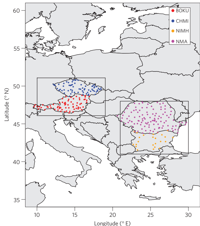
Figure 1 | Station observations and analysis domains. Location of high-density station observations from the CECILIA climate and extreme database (responsible institutions: University of Natural Resources and Life Sciences (BOKU), Austria; Czech Hydrometeorological Institute (CHMI), Czech Republic; National Institute of Meteorology and Hydrology (NIMH), Bulgaria; National Meteorological Administration (NMA), Romania), as well as analysed central and southeast European domains (boxes).
