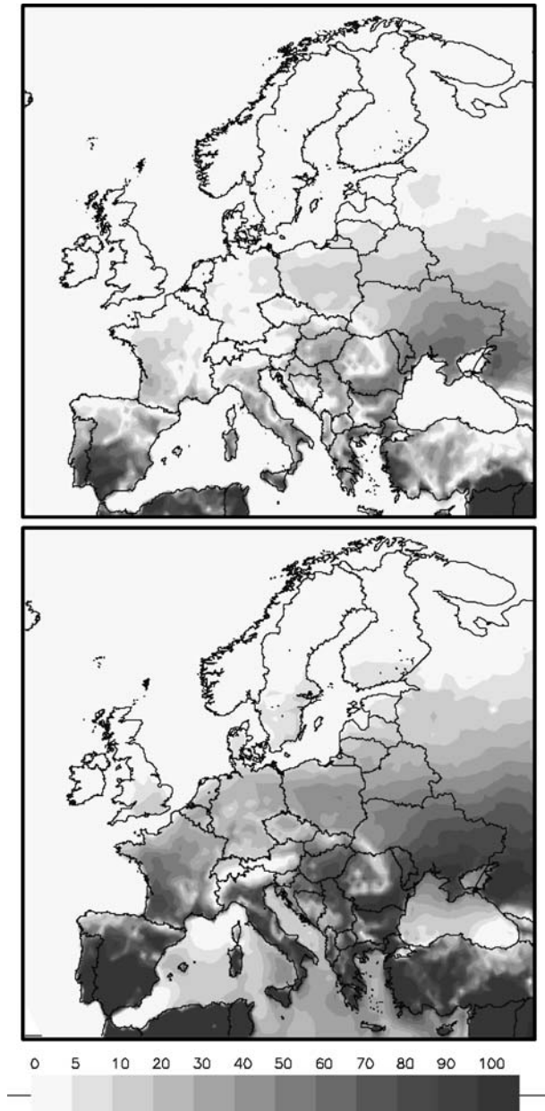
Fig. 2 Mean annual number of days above 30°C simulated by the HIRHAM4 regional climate model for the 1961–1990 ( upper ) and 2071–2100 ( lower ) periods
