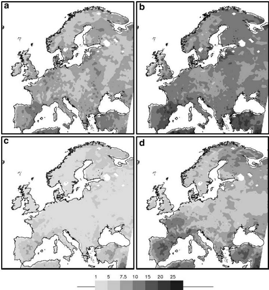
Fig. 3 Changes (expressed as a ratio) in the heat wave indices N_HW (a), HW_F (b), HW_D (c) and HW_I (d) between the 1961–1990 and 2071–2100 periods, based on HIRHAM4 simulations. (See text for details and definitions of these indices)
